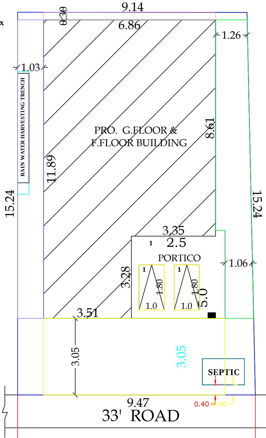
SITE PLAN
