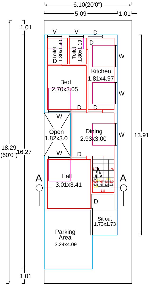
PLAN - G.F ( Facing SOUTH)
