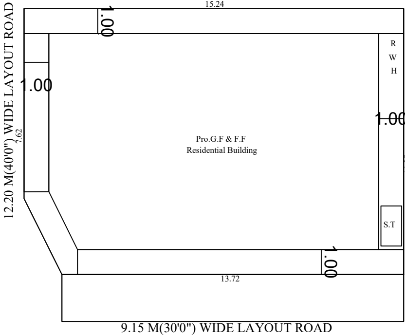
SITE PLAN
