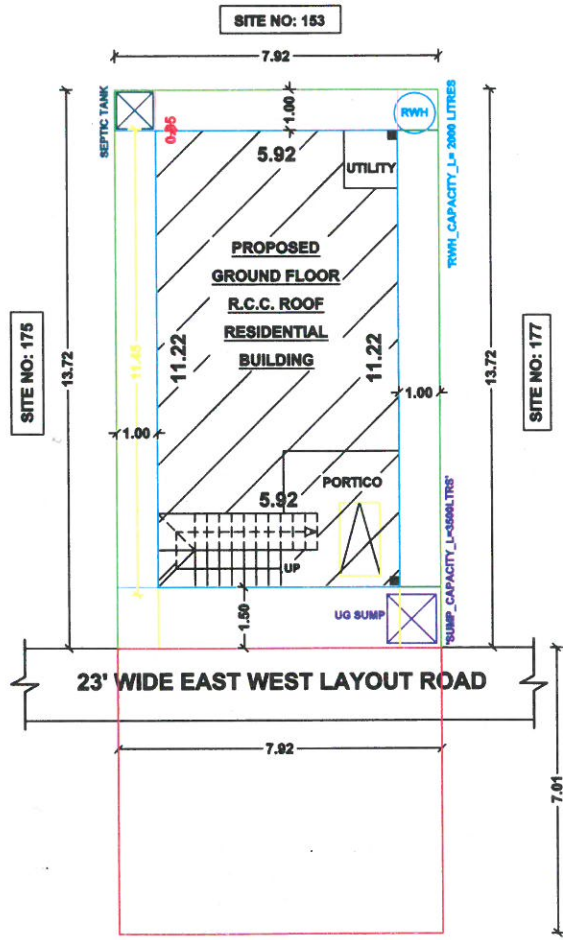
SITE PLAN
