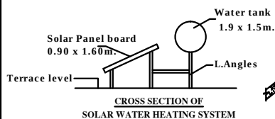
CROSS SECTION OF SOLAR WATER HEATING SYSTEM
