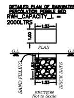
DETAILED PLAN OF RAINWATER DISPOSAL SYSTEM WITH RW CAPACITY 1.1 = 2000LTRS
