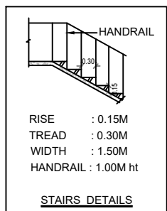
STAIRS DETAILS
