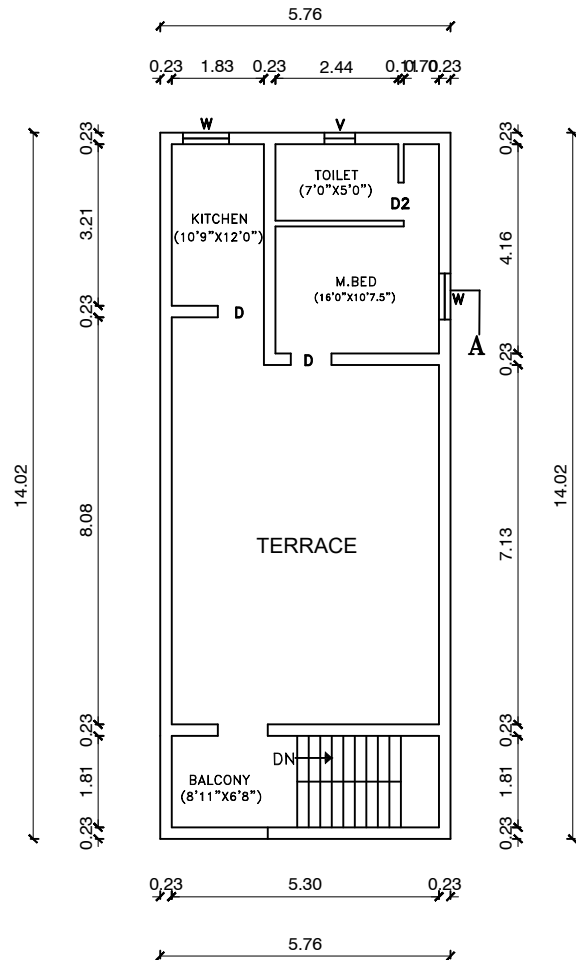
PROPOSED FIRST FLOOR PLAN (ADDITIONL)
