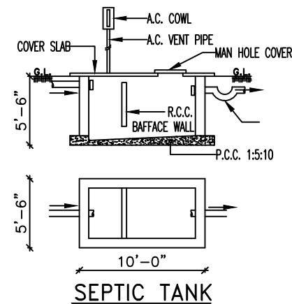
SEPTIC TANK
