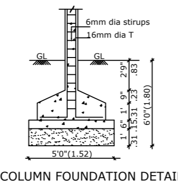
COLUMN FOUNDATION DETAIL
