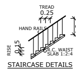
STAIRCASE DETAILS
