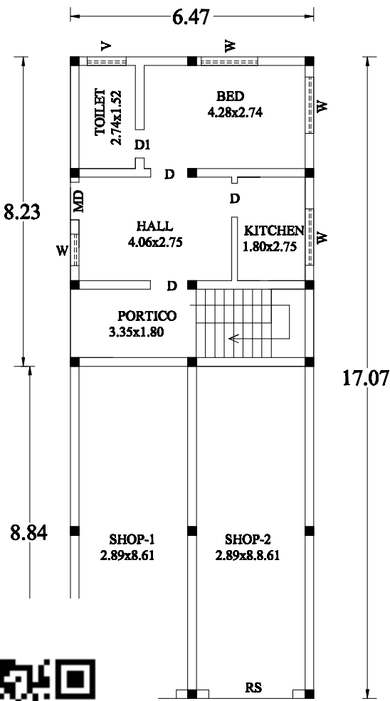
ND FLOOR
