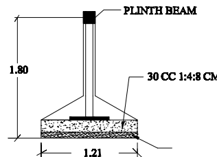
COLUMN DETAILS
