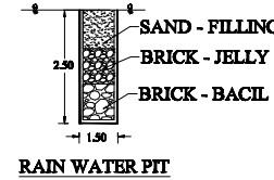
RAIN WATER PIT
