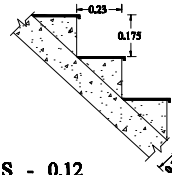
DETAIL OF STAIRCASE
