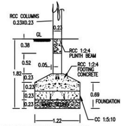
FOUNDATION DETAILS
