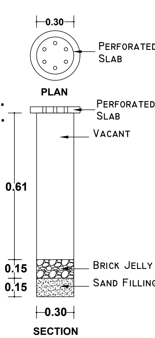
RAINWATER PERCOLATION PIT @ 3M INTERVAL
