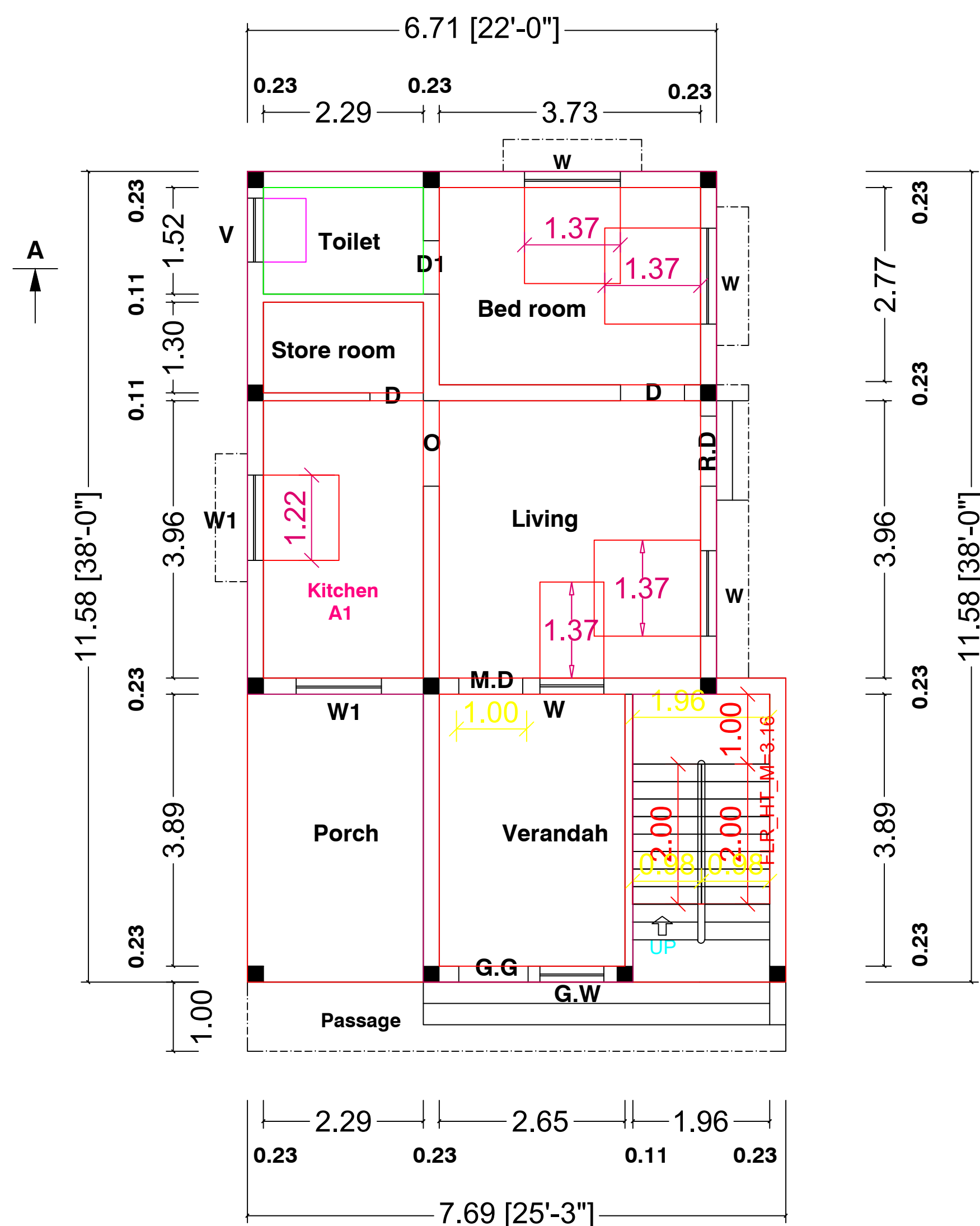
FLOOR-GROUND PLAN ( FACING NORTH )
