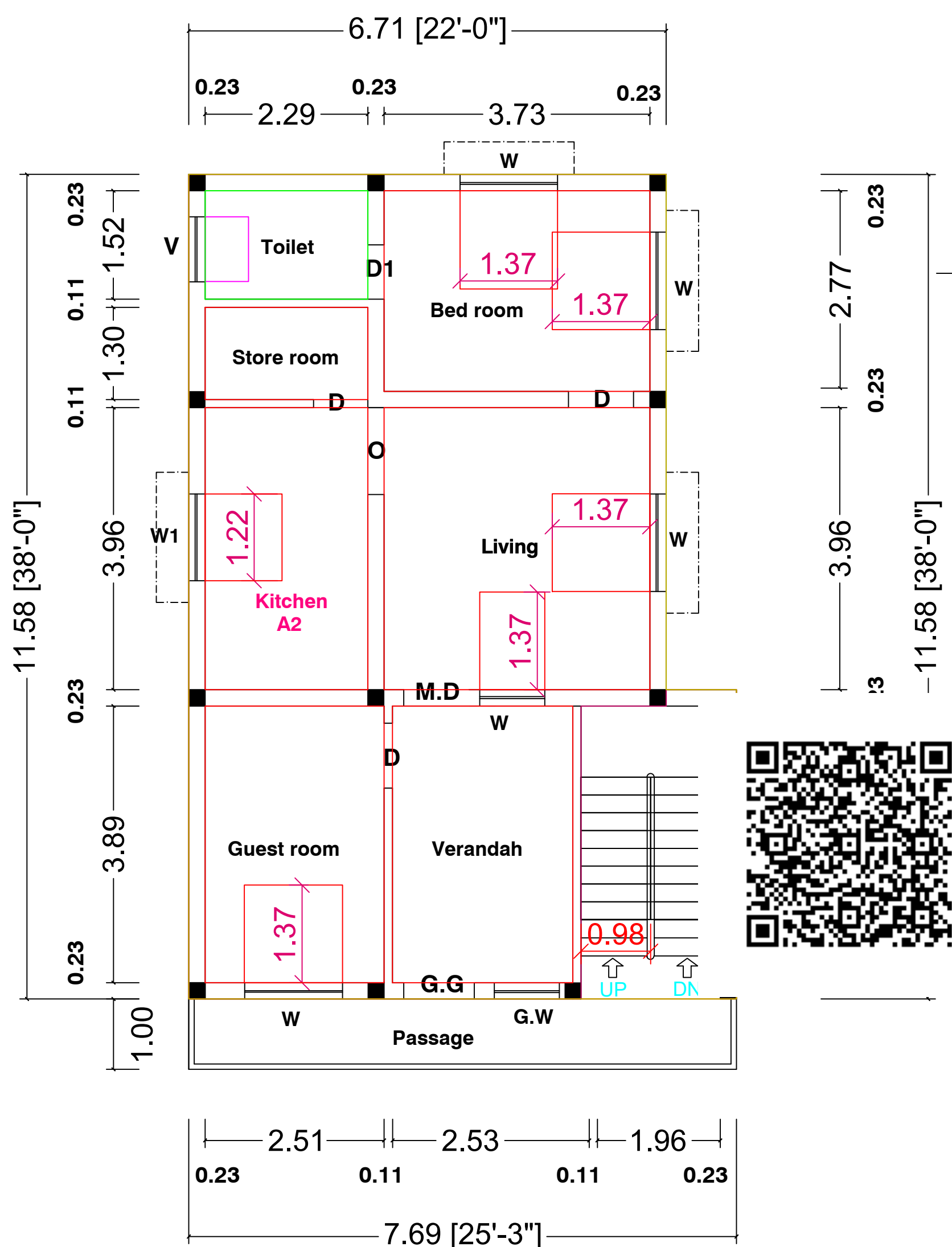
FLOOR01 PLAN ( FACING NORTH )
