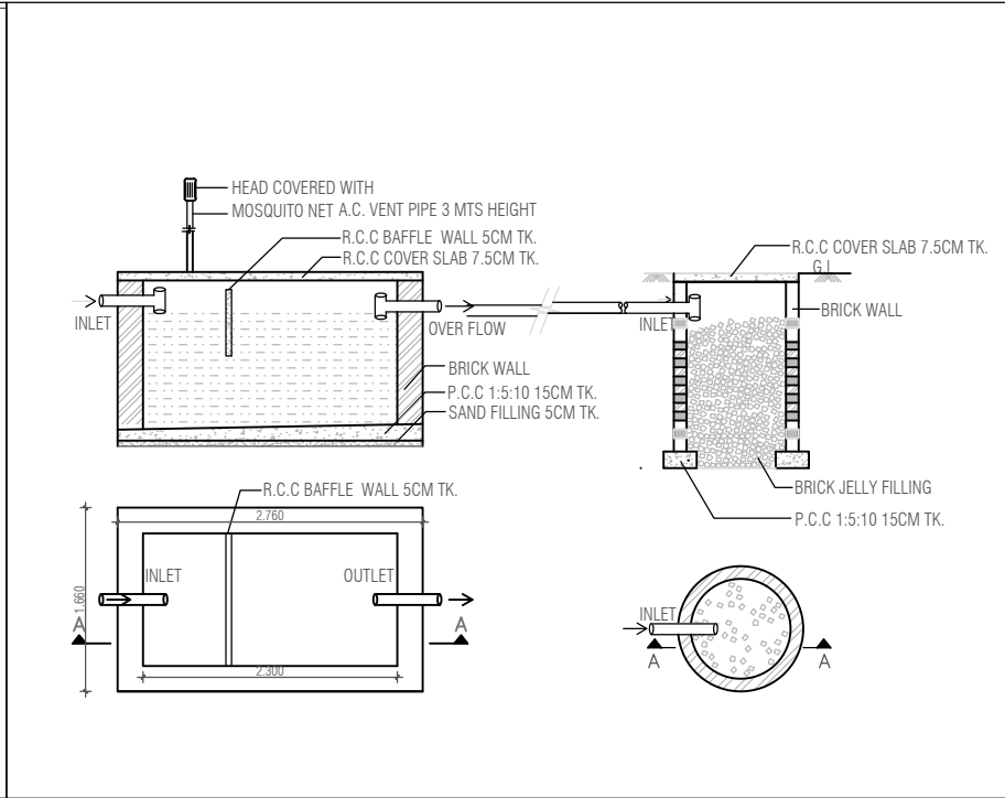
SEPTIC TANK DETAIL
