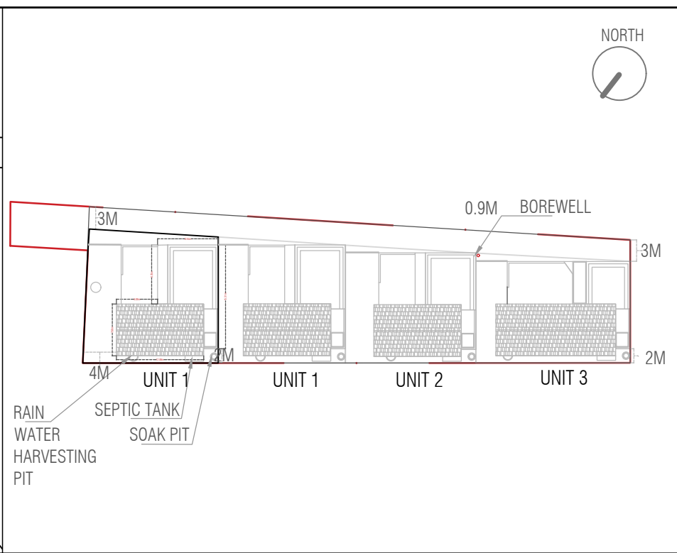
SITE PLAN
