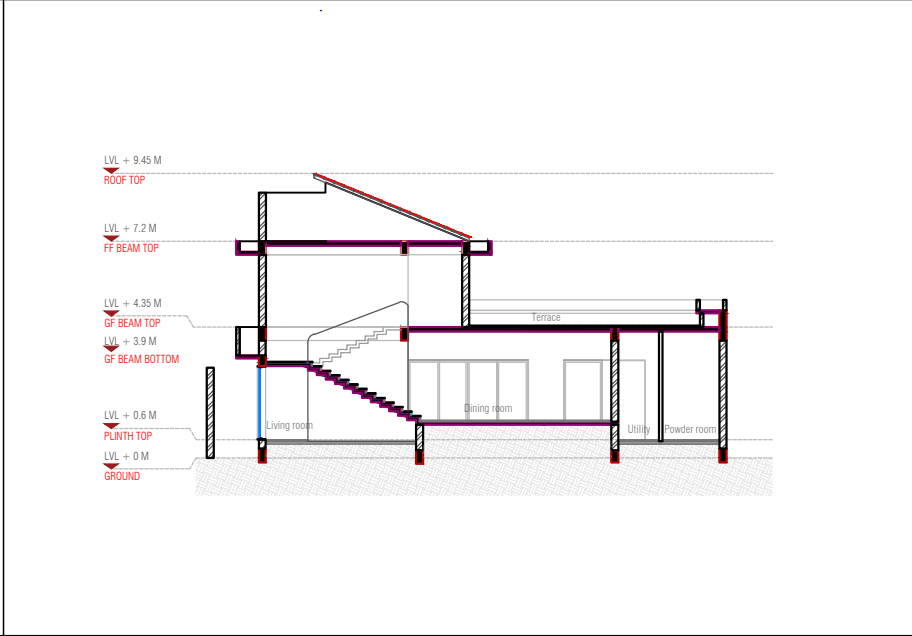
UNIT 1 SECTION BB'
