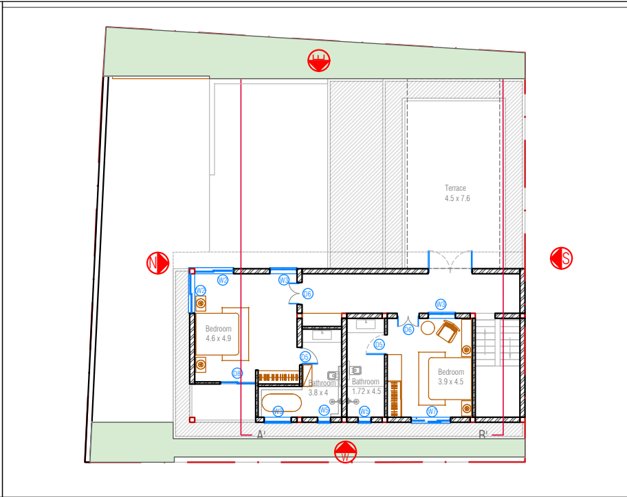
UNIT 1 FIRST FLOOR PLAN
