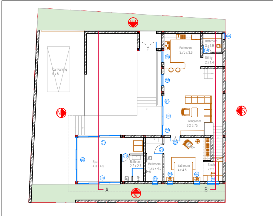
UNIT 1 GROUND FLOOR PLAN
