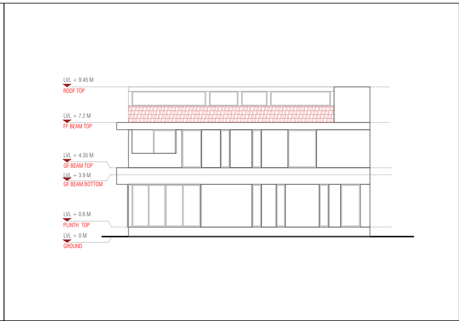
UNIT 1 WEST ELEVATION
