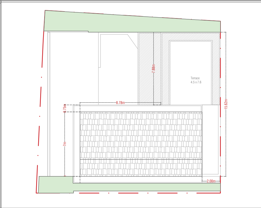
Unit 1 ROOF PLAN
