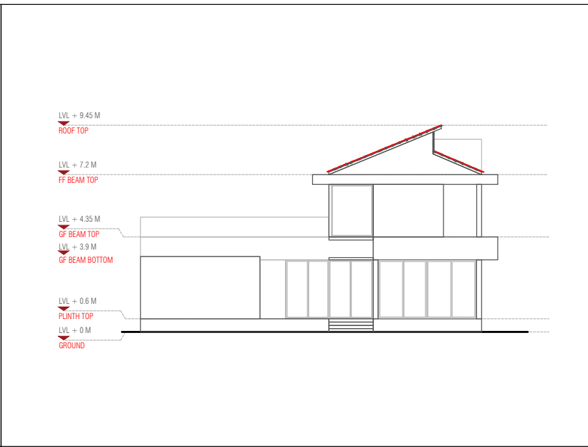
UNIT 1 NORTH ELEVATION
