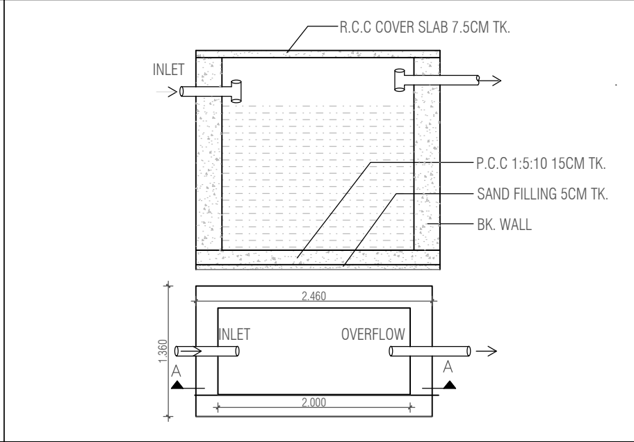
STORAGE PIT DETAIL
