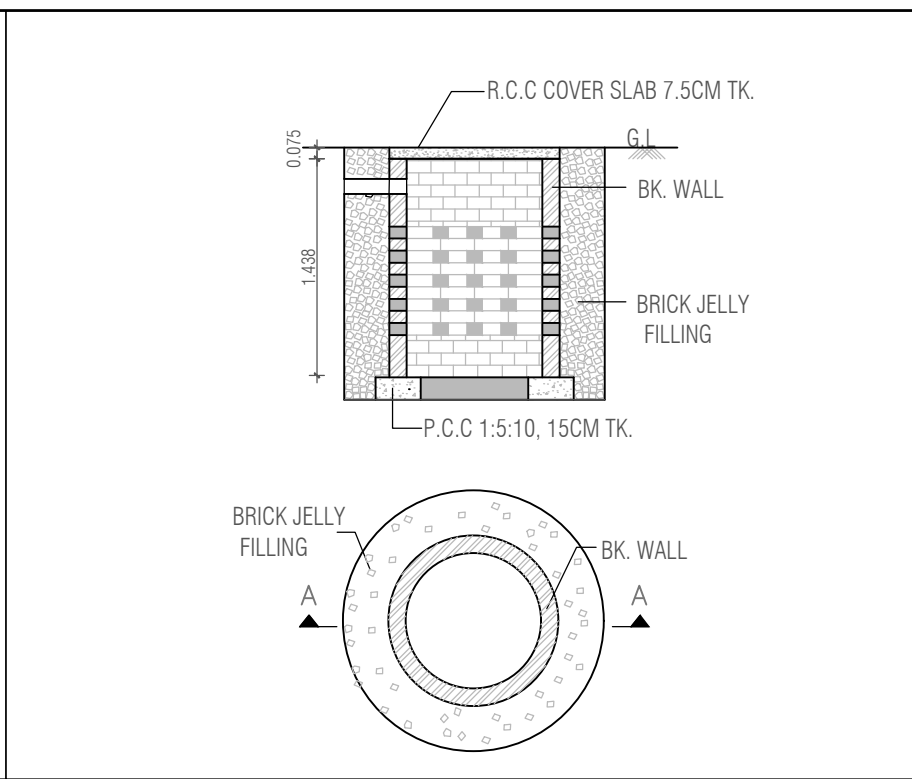
SOAK PIT DETAIL
