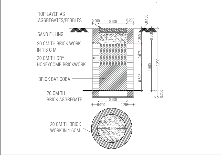
RAIN WATER HARVESTING PIT DETAIL
