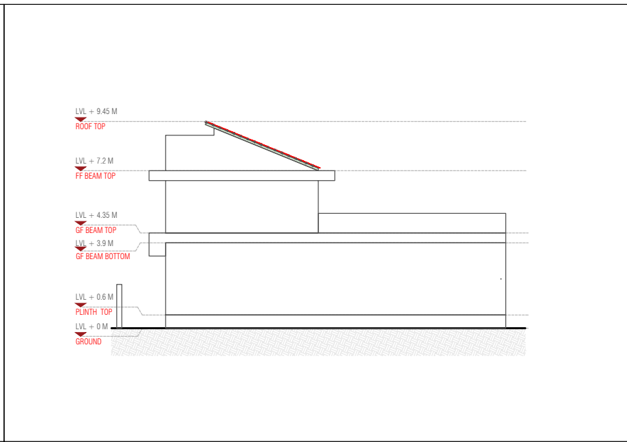
UNIT 1 SOUTH ELEVATION
