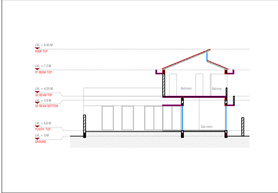
UNIT 1 SECTION AA'
