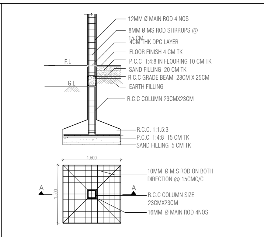
RCC FOUNDATION DETAIL
