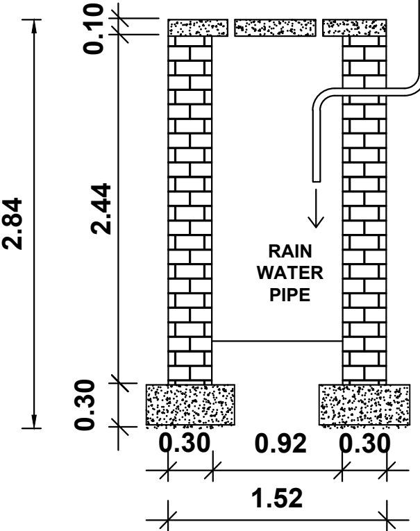
RAIN WATER HARVESTING NOT TO SCALE
