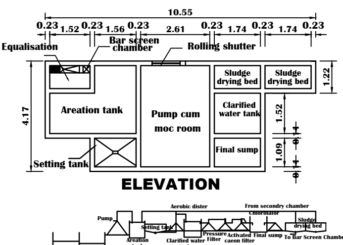
PLAN SEWAGE TREATMENT PLANT
