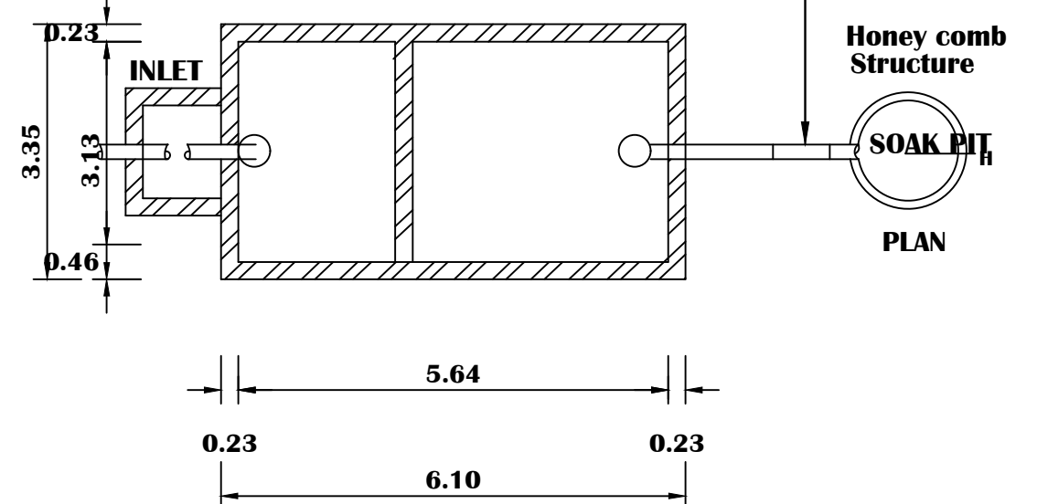
SEPTIC TANK PLAN SCALE 1:100
