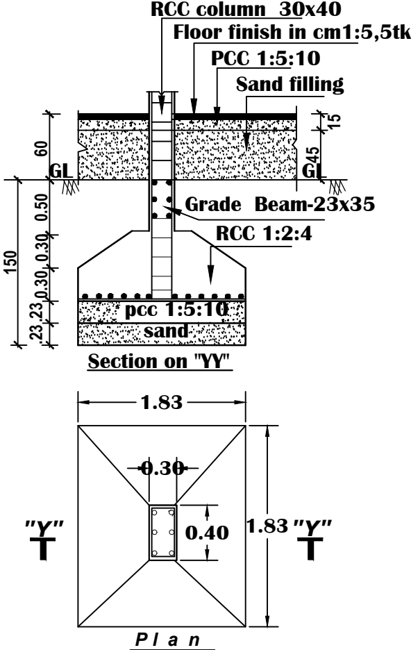
FOUNDATION DTLS (Scale 1:50)
