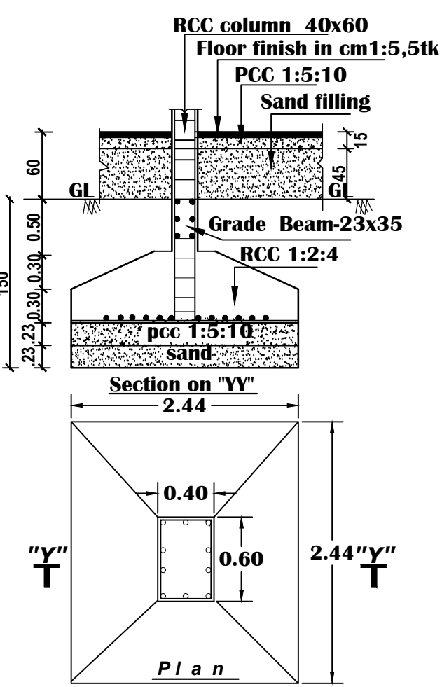
FOUNDATION DTLS (Scale 1:50)
