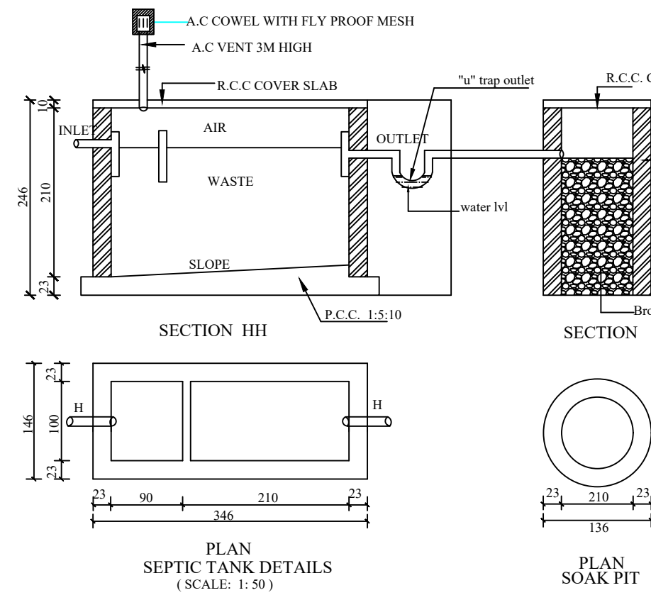
PLAN SEPTIC TANK DETAILS (SCALE: 1:50)
