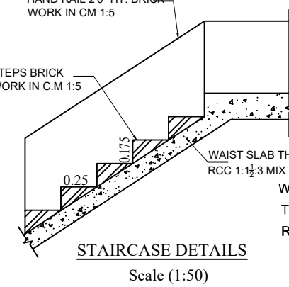
STAIRCASE DETAILS Scale (1:50)
