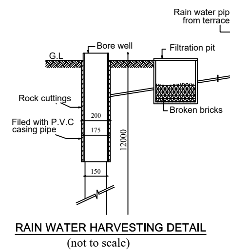
RAIN WATER HARVESTING DETAIL (not to scale)
