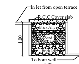
RAIN WATER HARVEST PIT
