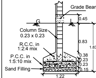
FOUNDATION DETAILS Scale 1:75
