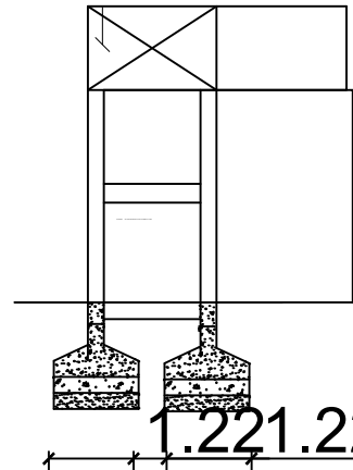
SECTION OF WATER TANK
