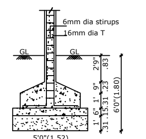
COLUMN FOUNDATION DETAIL SCALE (1:50)
