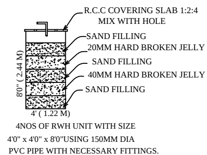
RAIN WATER HARVEST UNIT
