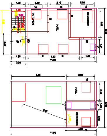
GROUND FLOOR PLAN FIRST FLOOR PLAN
