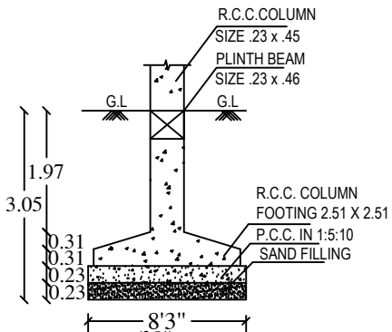
FOUNDATION DETAIL
