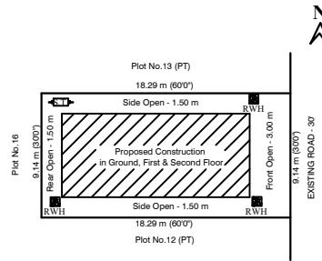
SITE PLAN
