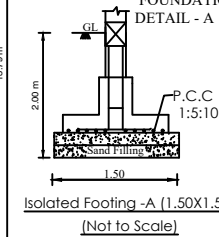
SECTION - 'CD'
