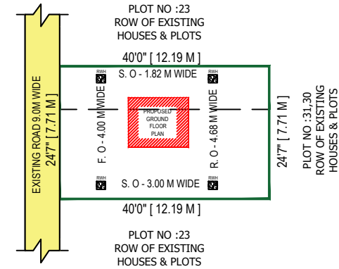
SITE PLAN SCALE - 1:200
