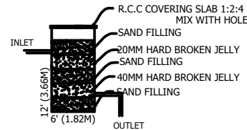
WASTE WATER RECYCLE UNIT
