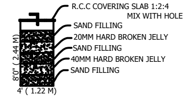
RAIN WATER HARVEST UNIT
