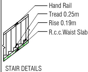
STAIR DETAILS
