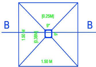
FOUNDATION DETAILS
