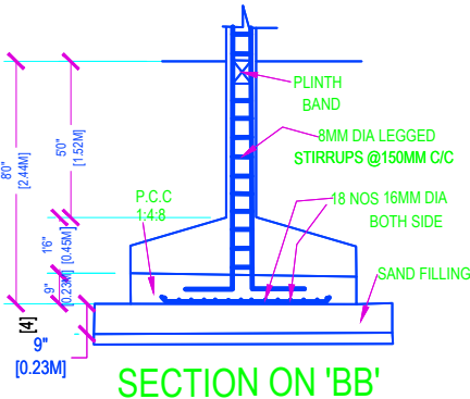
SECTION ON "BB"
