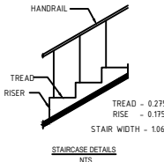
STAIRCASE DETAILS
