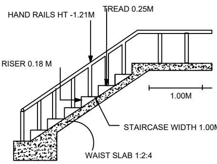
STAIRCASE DETAILS
