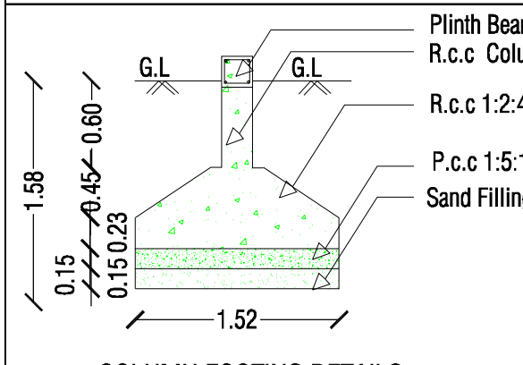
COLUMN FOOTING DETAILS
