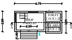
PRO. GROUND FLOOR PLAN
