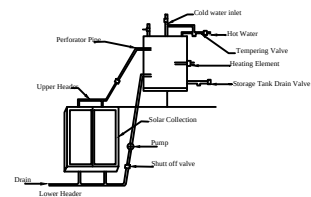
Details Of Solar Water Heater (NTS)
