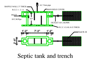
Septic tank and trench
