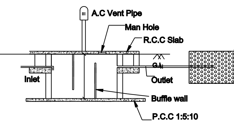
SECTION PLAN OF SEPTIC TANK & TRENCH
