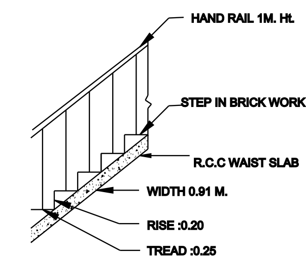
STAIR DETAIL
