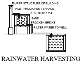
RAINWATER HARVESTING
