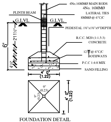
FOUNDATION DETAIL
