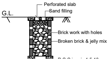
RAINWATER HARVESTING
