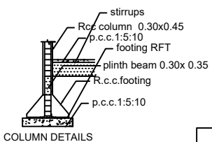
COLUMN DETAILS
