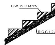
STAIRCASE
