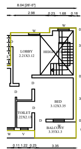
FLOOR PLAN
