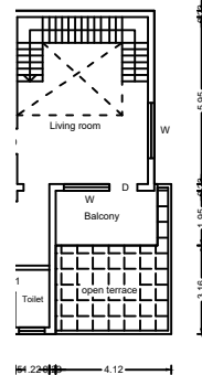
FLOOR PLAN
