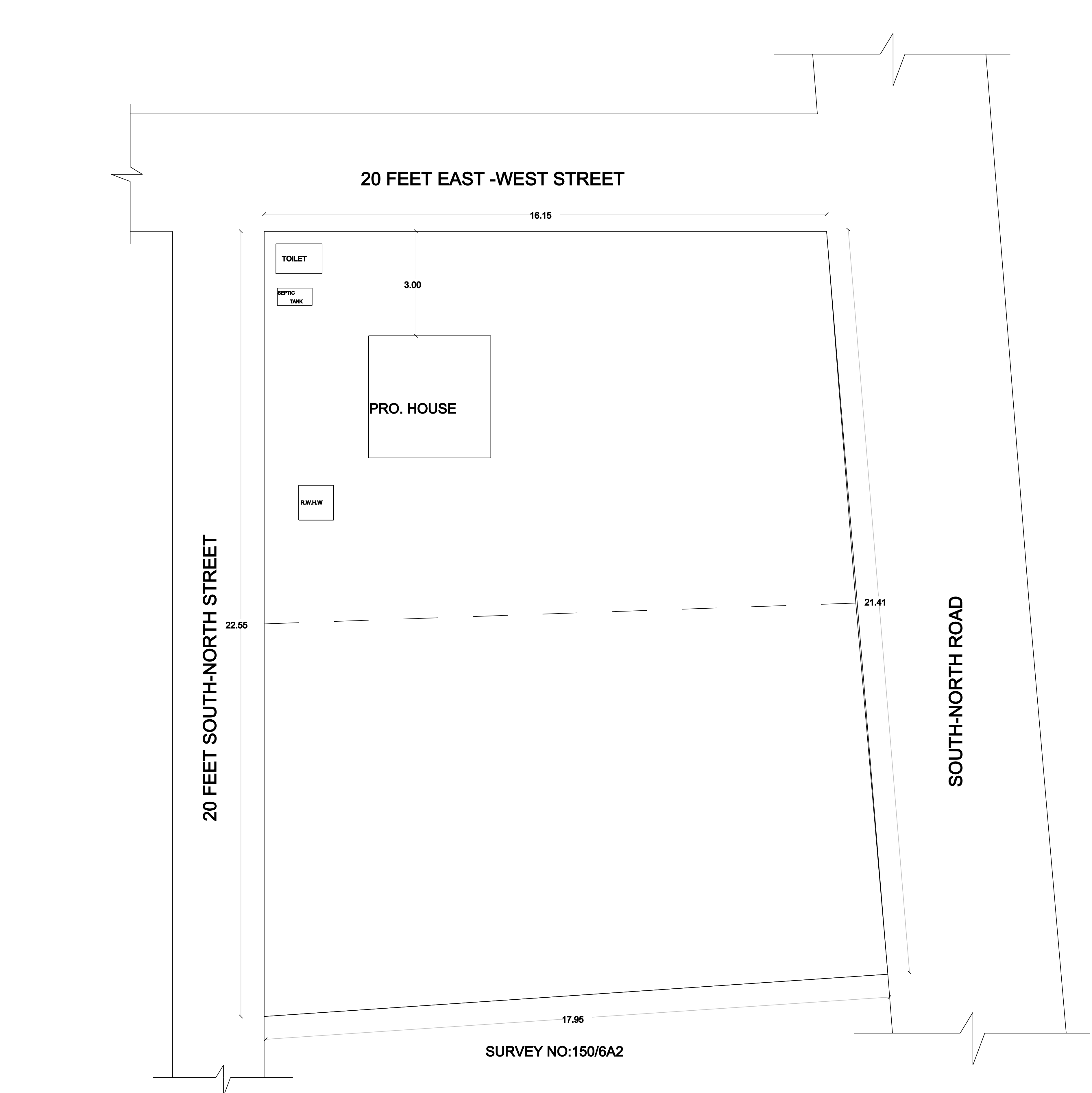
SITE PLAN
