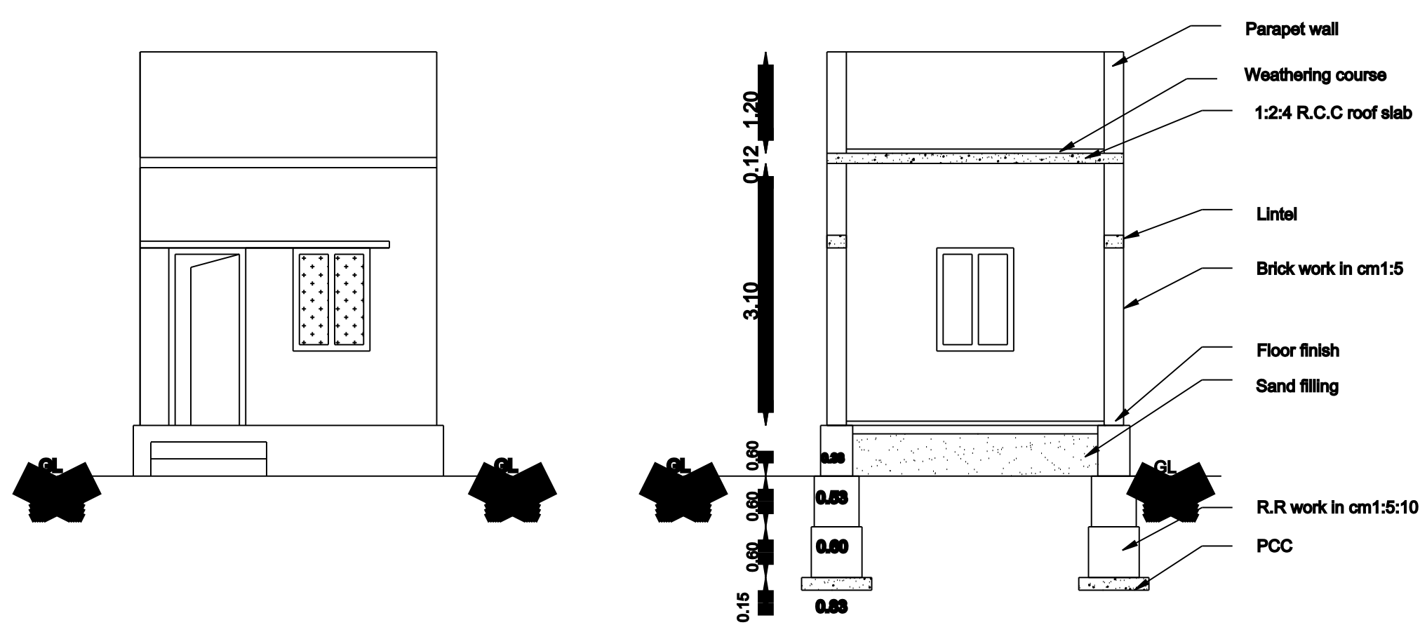
FRONT ELEVATION
