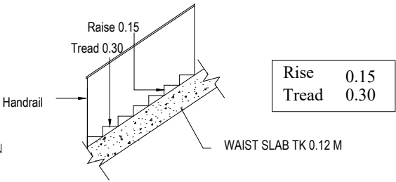
STAIRCASE DETAIL
