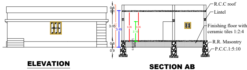
SECTION AB
