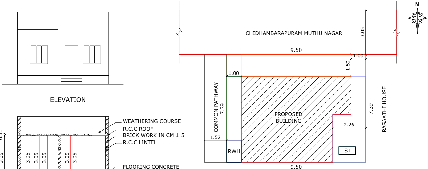
ELEVATION CHIDHAMBARAPURAM MUTHU NAGAR PROPOSED BUILDING COMMON PATHWAY RASAATHI HOUSE THAVASIKANI SITE SITE PLAN SCALE - 1:100
