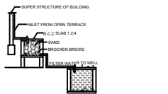
DETAILS OF FILTER BED & WELL NTS
