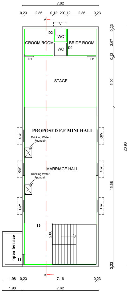
FIRST FLOOR PLAN PROPOSED
