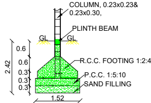
COLUMN DETAILS
