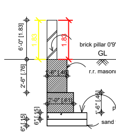
COMPOUND WALL DETAIL scale: 0'1" = 4'0"
