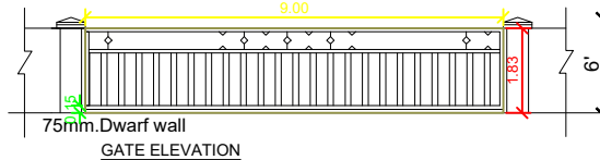
GATE ELEVATION
