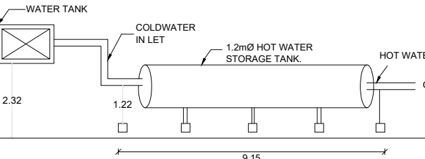
SOLAR WATER HEATING SWHS DETAIL
