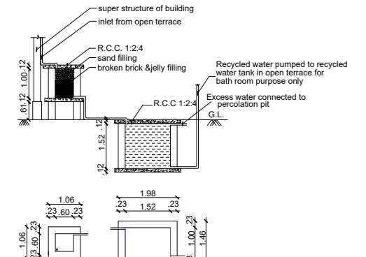
Sump and Filter Bed
