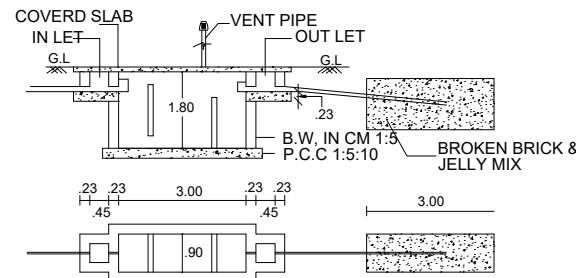
PLAN & SECTION OF SEPTIC TANK & TRENCH
