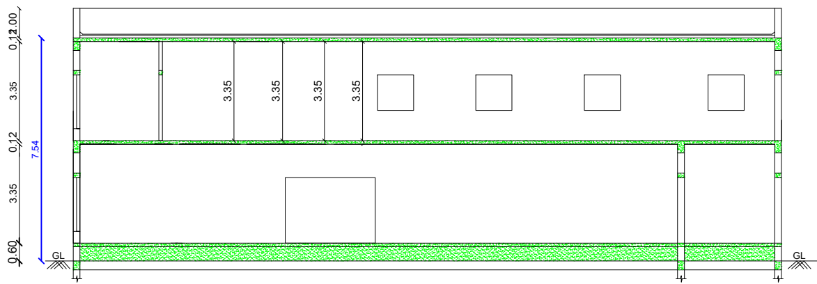
SECTION ON AB & (HALF ELEVATION)
