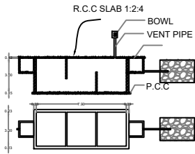
SEPTIC TANK AND TRENCH NTS
