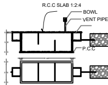
SEPTIC TANK AND TRENCH NTS
