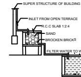
DETAILS OF FILTER BED & WELL NTS
