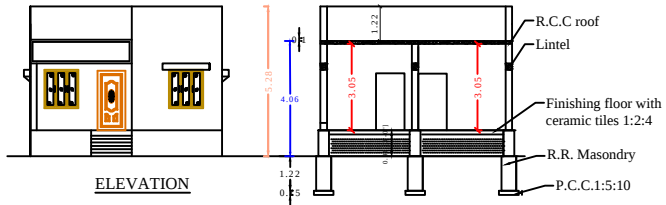
SECTION AB
