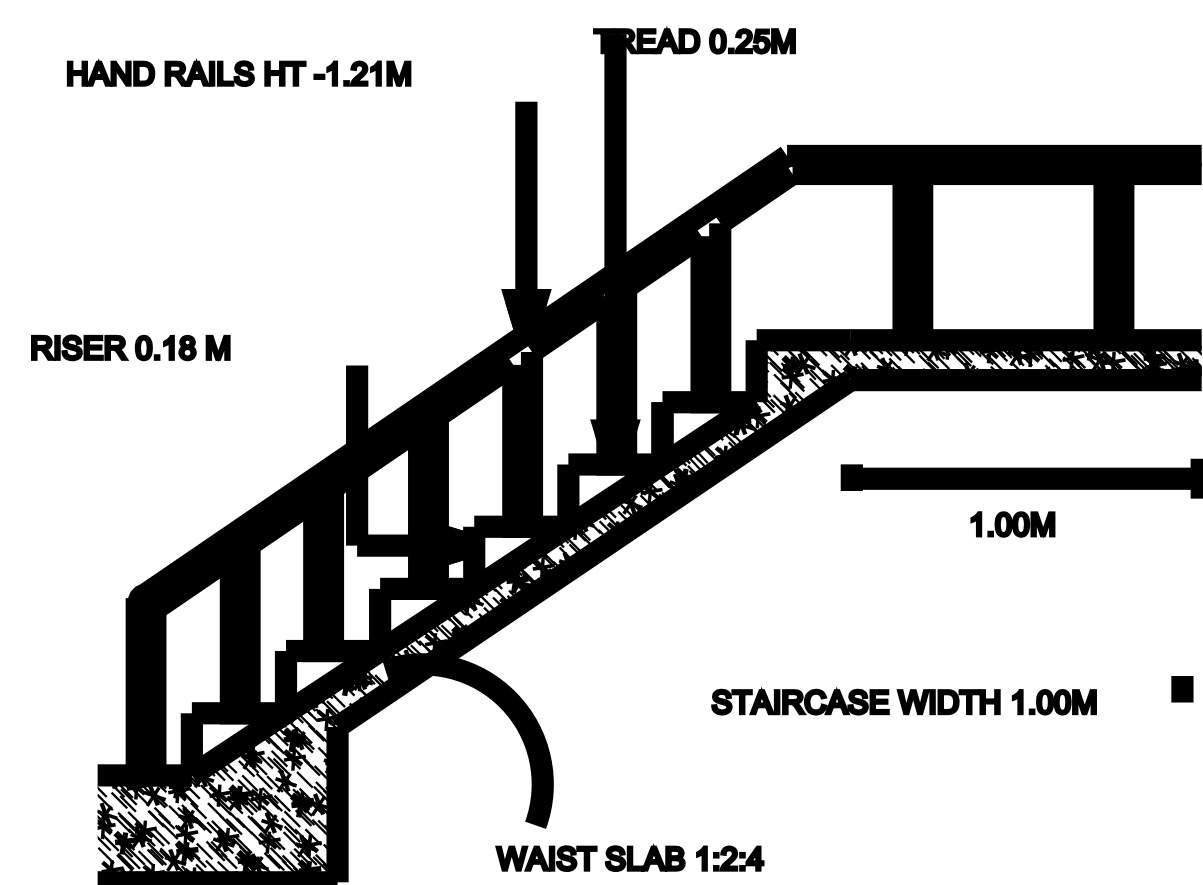
STAIRCASE DETAILS
