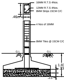
RCC COLUMN DETAILS
