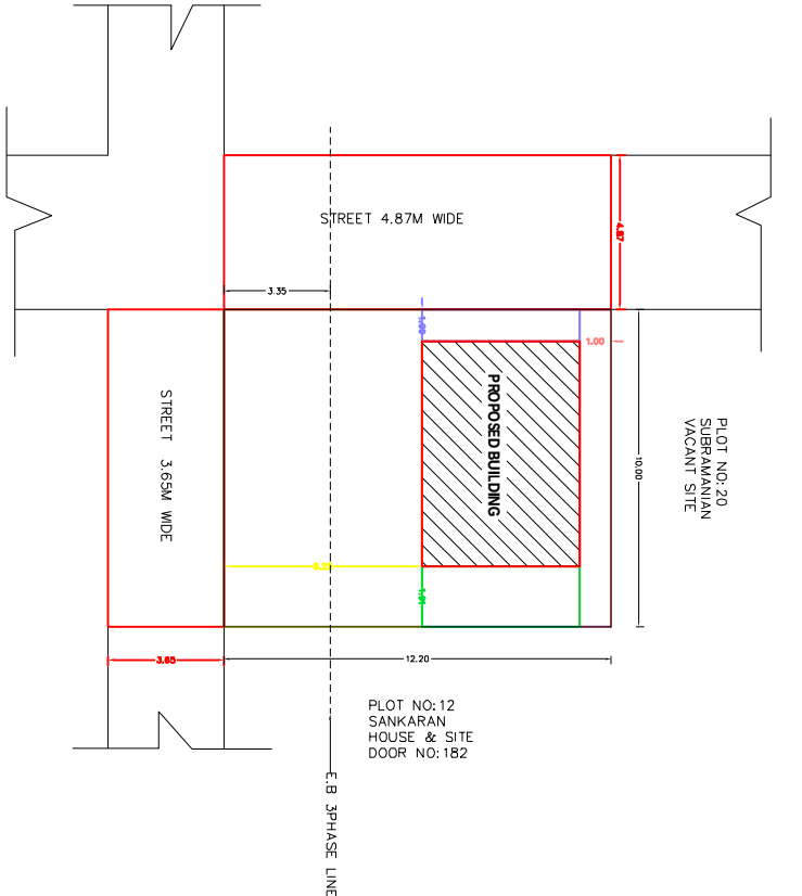
SITE PLAN (Scale 1:100CM)
