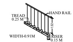
STAIRCASE DETAILS
