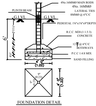
FOUNDATION DETAIL
