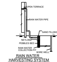
RAIN WATER HARVESTING SYSTEM
