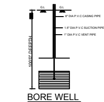
BORE WELL
