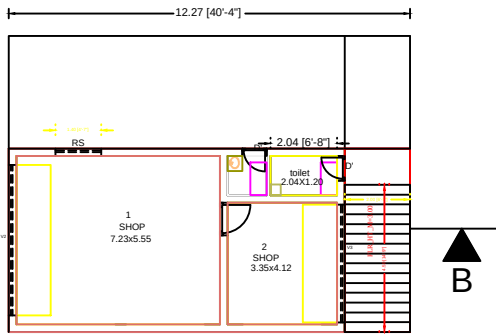
FIRST FLOOR PLAN FLOOR-FIRST
