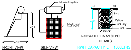
SOLAR WATER HEATER DETAILS (SCALE 1:100)
