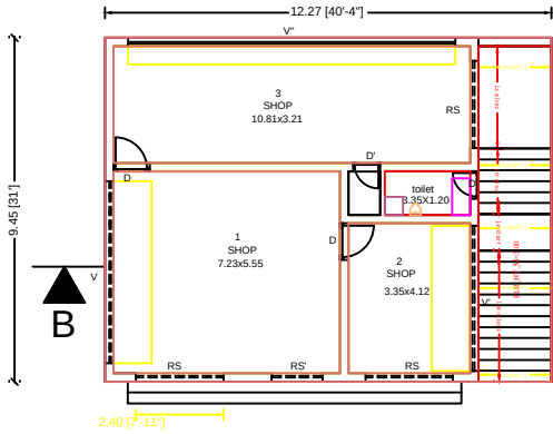
GROUND FLOOR PLAN FLOOR-GROUND
