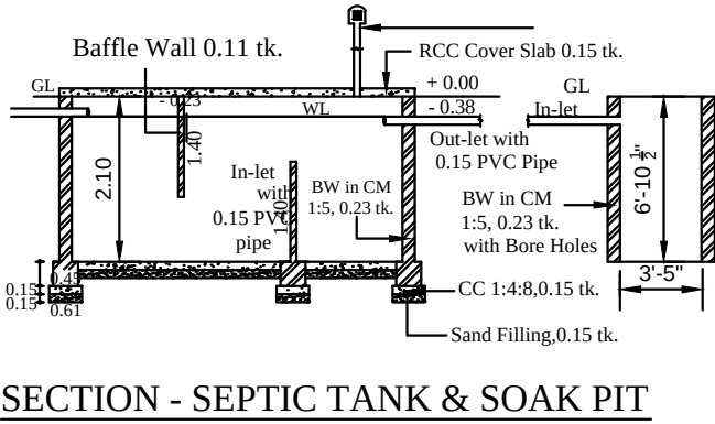
SECTION - SEPTIC TANK & SOAK PIT
