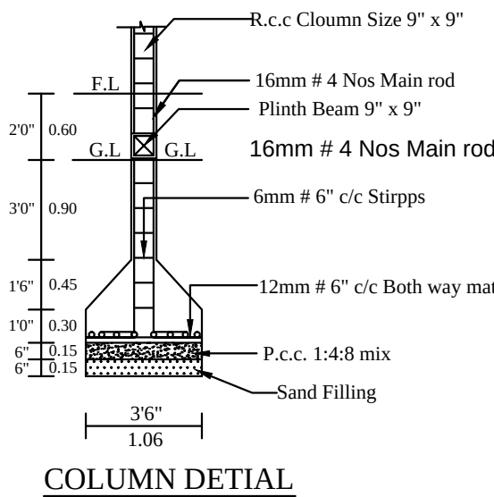
COLUMN DETIAL
