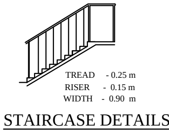
STAIRCASE DETAILS
