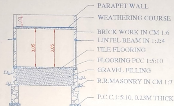
SECTION ON "V-B"
