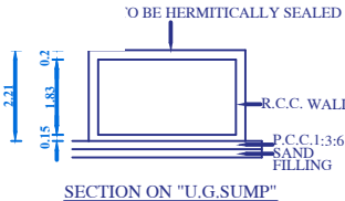
SECTION ON "U.G.SUMP"
