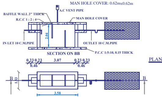
SEPTIC TANK AND TRENCH & U TRAP ADOPTED
