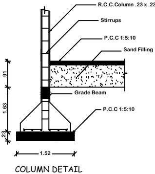
COLUMN DETAIL
