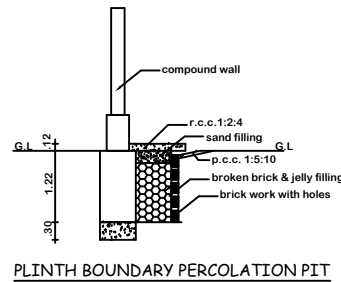
PLINTH BOUNDARY PERCOLATION PIT
